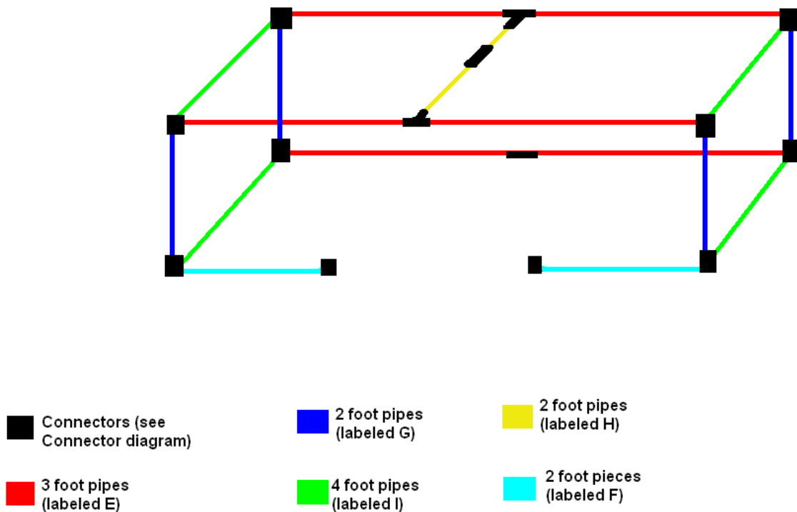
Figure 2. End chamber diagram
